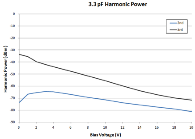
Figure 2. Harmonic Power
